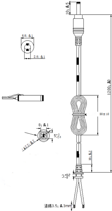
DC Cord Drawing
