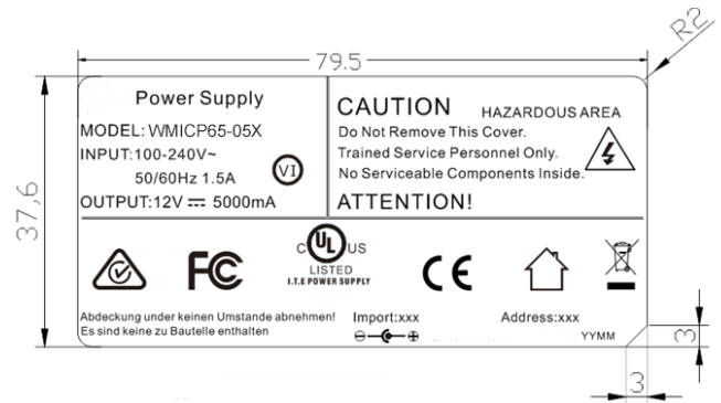
Label Drawing
