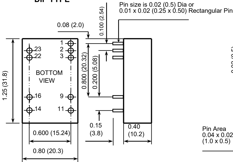
(DIP) PIN CONNECTION
