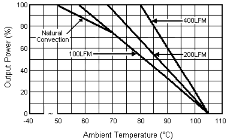
DERATING CURVE
