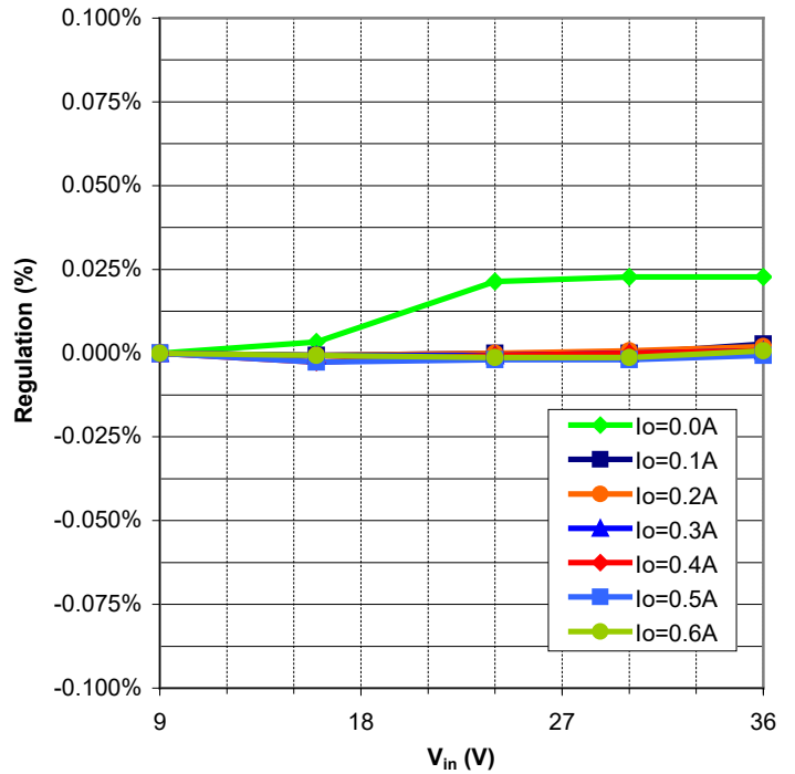
Graph 7: Line Regulation
