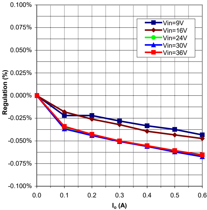
Graph 6: Load Regulation
