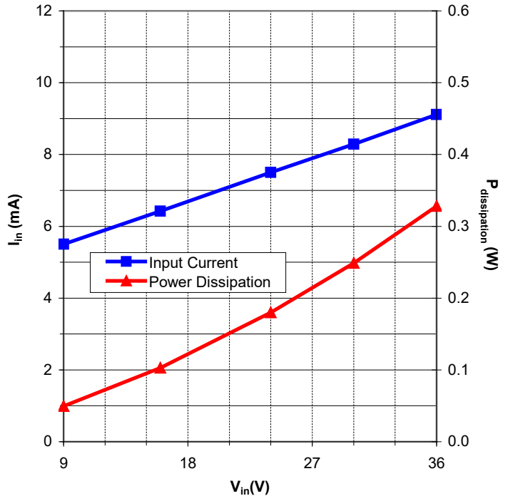
Graph 6: 'Remote Off' Input Current and Power Dissipation vs. Input Voltage
