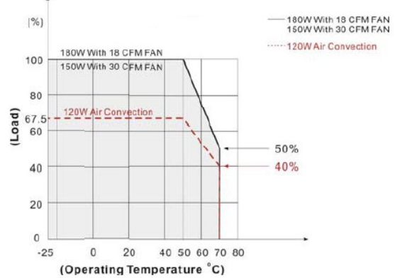
Power Derating Curve for U-Chassis & Enclosed Models
