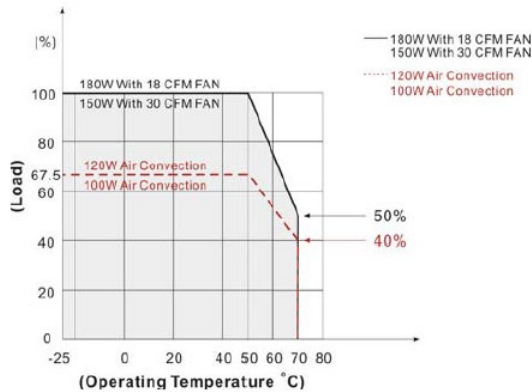
Power Derating Curve for Open Frame Models
