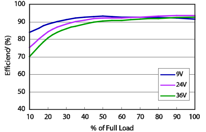
DHW24S15-50 Efficiency vs Load Current
