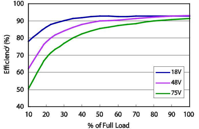
DHW48S15-50 Efficiency vs Load Current
