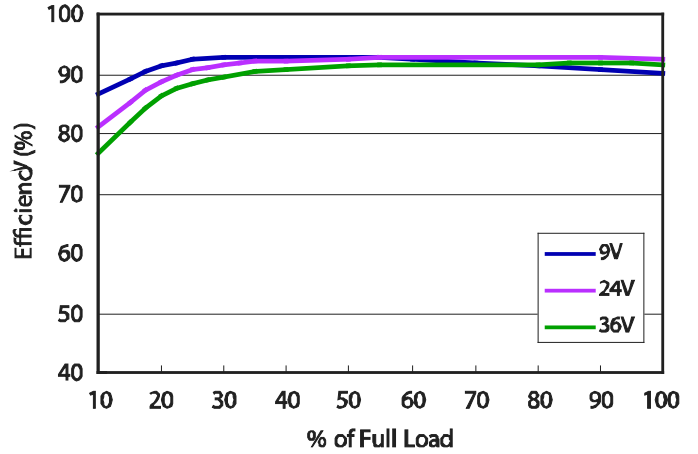
DHW24S5-50 Efficiency vs Load Current
