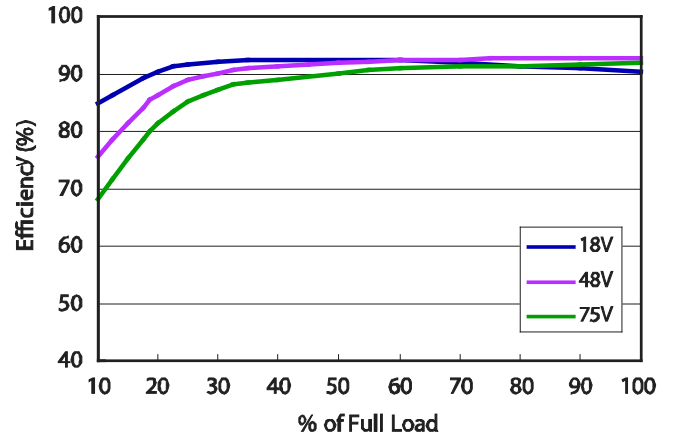
DHW48S5-50 Efficiency vs Load Current
