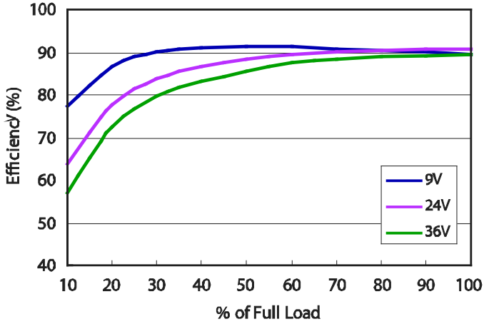
DHW24S3.3-33 Efficiency vs Load Current
