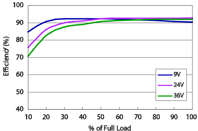
DHW24S24-50 Efficiency vs Load Current
