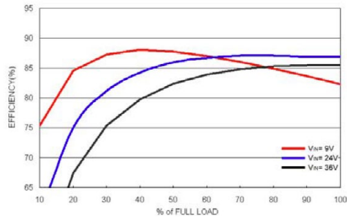
Efficiency vs. Output Load
