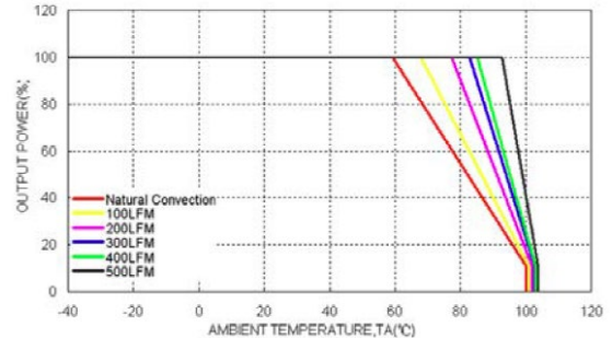
Derating Output Load vs. Ambient Temp. & Airflow V_{in} = V_{in}(\text{nom})
