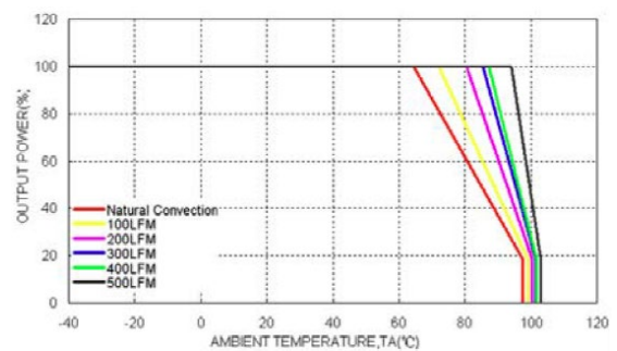
Derating Output Load vs. Ambient Temp. & Airflow V_{in} = V_{in}(\text{nom})
