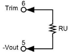
Trim Up
