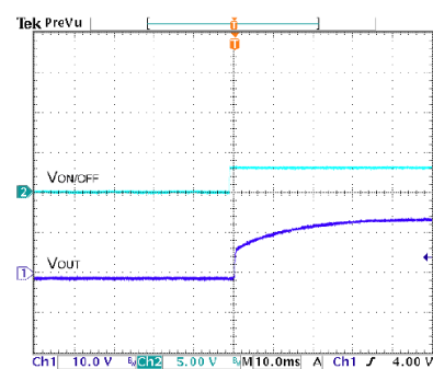
Using ON/OFF Voltage Start-Up and V_{out} Rise Characteristic V_{in} = V_{in}(\text{nom}) , Full Load
