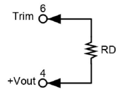
Trim Down
