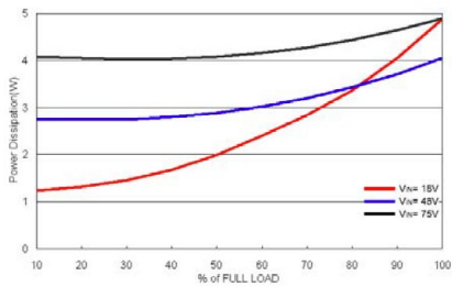
Power Dissipation vs. Output Load
