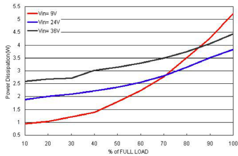
Power Dissipation vs. Output Load
