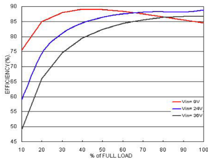
Efficiency vs. Output Load
