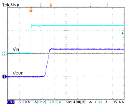
Typical Input Start-Up & Output Rise Characteristic V_{in} = V_{in}(\text{nom}) , Full Load
