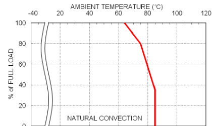
Derating Curve with Heatsink
