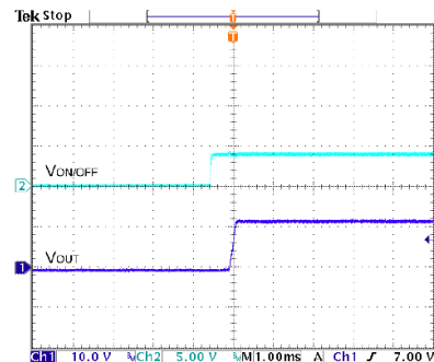
Using ON/OFF Voltage Start-Up and V_{out} Rise Characteristic V_{in} = V_{in}(\text{nom}) , Full Load
