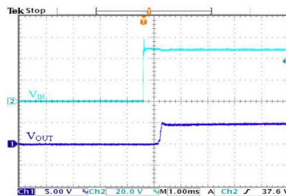
Typical Input Start-Up & Output Rise Characteristic, Vin=Vin(nom), Full Load
