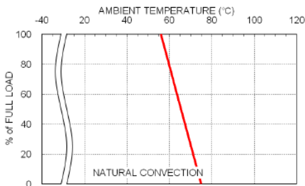
Derating Curve
