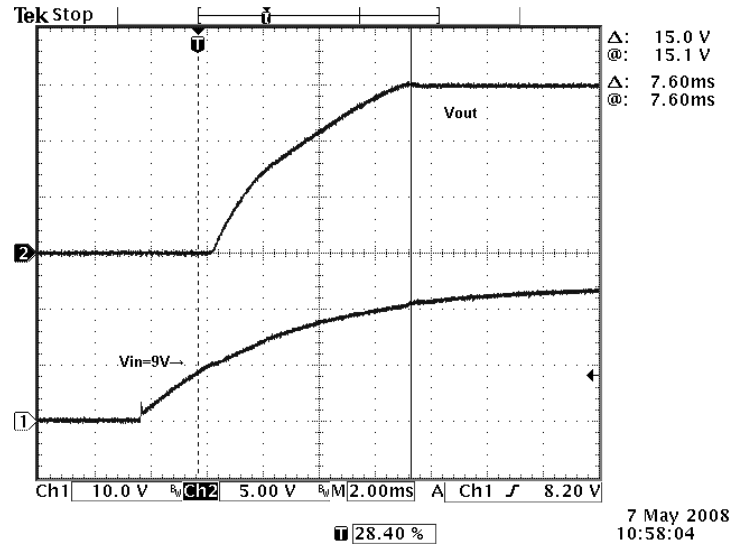
Photo 6: Turn On at Full Load V_{in} = 24 \text{ Vdc} ; I_{out} = 0.533 \text{ A} C_{out} = 680 \mu\text{F} Aluminum Electrolytic
