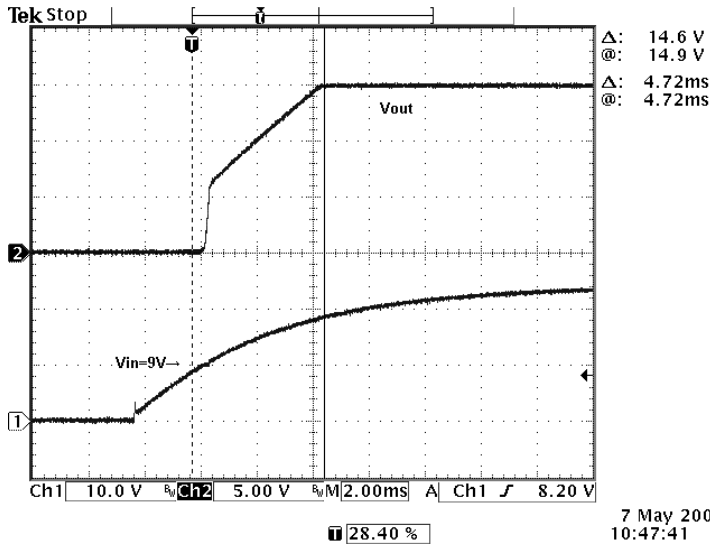
Photo 5: Normal Turn On at No Load V_{in} = 24 \text{ Vdc} ; I_{out} = 0 \text{ A}
