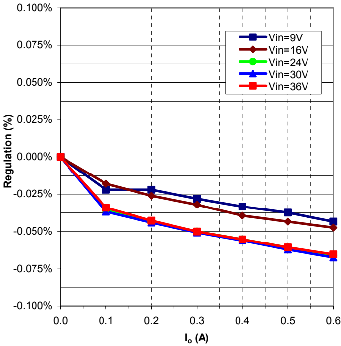
Graph 6: Load Regulation
