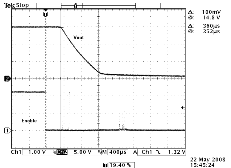
Photo 8: Turn Off by Enable V_{in} = 24 \text{ Vdc} ; I_{out} = 0.533 \text{ A}
