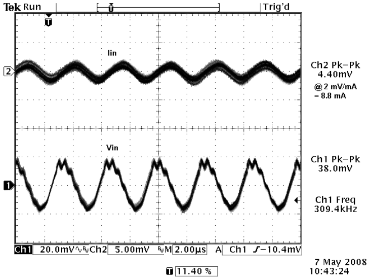
Photo 1: Input Ripple Voltage and Current V_{in} = 24\text{ V} , I_{out} = 0.533\text{ A} With a 1\ \mu\text{F} Ceramic across the Input
