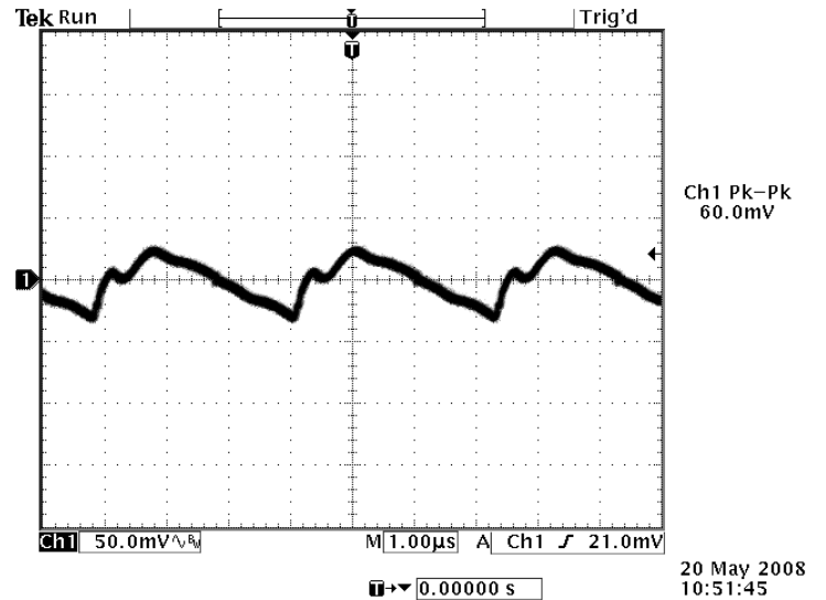
Photo 4: Output Ripple and Noise (20 MHz BW) V_{in} = 24\text{ V} , I_{out} = 0.533\text{ A} With a 1\ \mu\text{F} Ceramic across the Output
