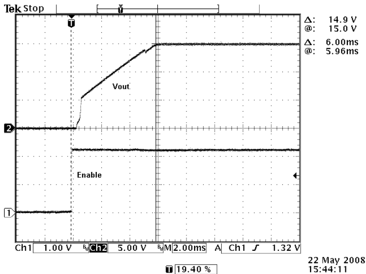
Photo 7: Turn On by Enable V_{in} = 24 \text{ Vdc} ; I_{out} = 0.533 \text{ A}
