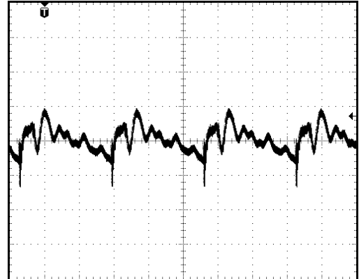
TYPICAL OUTPUT RIPPLE 50mV/div, 1uS/div, full load 75Vin 0.1uF decoupling cap at room temp
