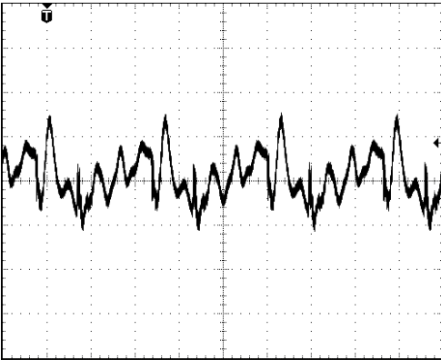
TYPICAL OUTPUT RIPPLE 20mV/div, 1uS/div, full load, 18Vin 0.1uF decoupling cap at room temp
