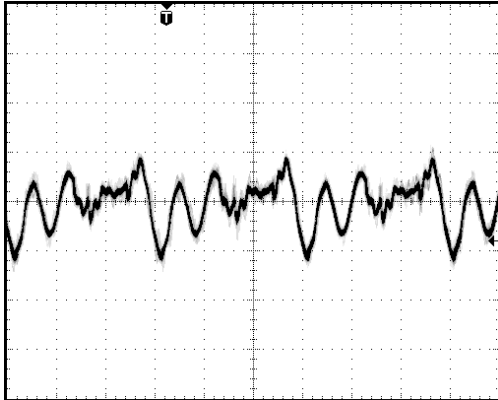
TYPICAL OUTPUT RIPPLE 50mV/div, 2 \mu S/div, full load, 18Vin 0.1 \mu F decoupling cap at room temp
