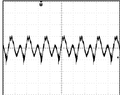
TYPICAL OUTPUT RIPPLE 50mV/div, 2 \mu S/div, full load 75Vin 0.1 \mu F decoupling cap at room temp
