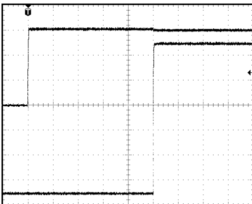
TYPICAL RISE TIME & TURN-ON DELAY USING LOGIC ENABLE 2V/div, 100mS/div (Vout), 2V/div 100mS/div (logic enable) 18Vin, full load at room temp
