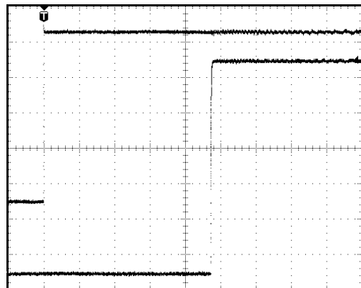
TYPICAL RISE TIME & TURN-ON DELAY WITH Vin 0-48V 2V/div, 100mS/div (Vout), 10V/div, 100mS/div (Vin) at room temp
