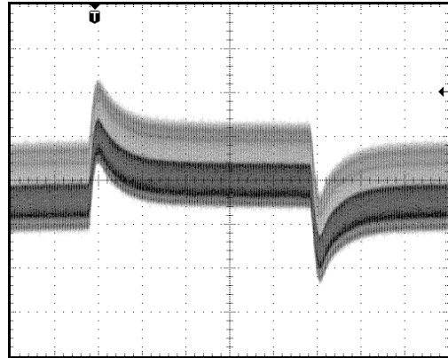
TYPICAL TRANSIENT RESPONSE 50mV/div, 200 \mu S/div, 50% full load to 75% full load 48Vin room temp
