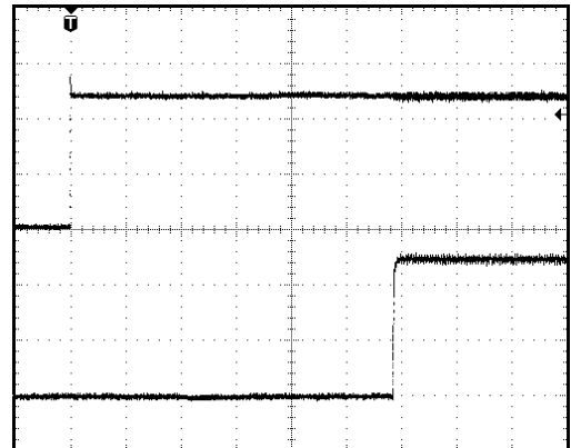
TYPICAL RISE TIME & TURN-ON DELAY WITH Vin 0-24V 2V/div, 40mS/div (Vout), 10V/div, 40mS/div (Vin) at room temp
