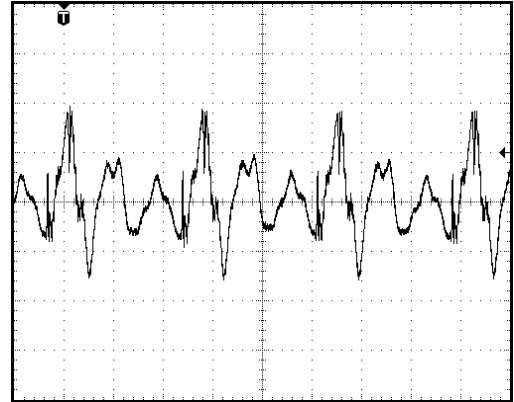
TYPICAL OUTPUT RIPPLE 20mV/div, 1uS/div, full load 36Vin 0.1uF decoupling cap at room temp
