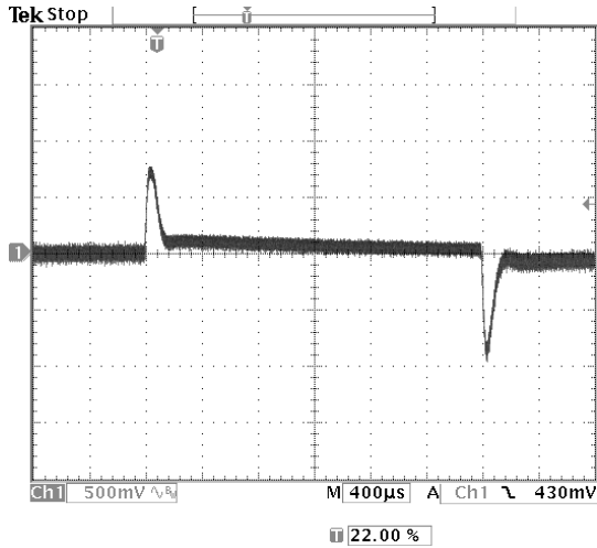
Photo 7: Transient Response 50% to 100% V_{in}=24V , I_{out} = 2.9 to 5.8A C_{out}=1\mu F Ceramic + 10\mu F Tantalum
