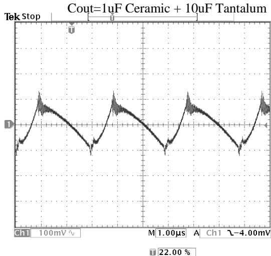
Photo 11: Output Voltage Ripple (Spike) V_{in}=24V , I_{out} = 5.8A C_{out}=1\mu F Ceramic + 10\mu F Tantalum
