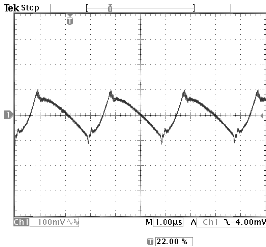
Photo 10: Output Voltage Ripple (20 MHz BW) V_{in}=24V , I_{out}=5.8A C_{out}=1\mu F Ceramic + 10\mu F Tantalum
