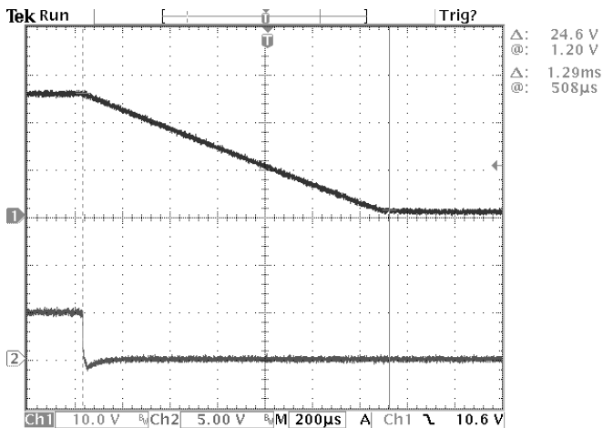
Photo 5: Remote Turn Off Vin=24V, Iout = 0.6A
