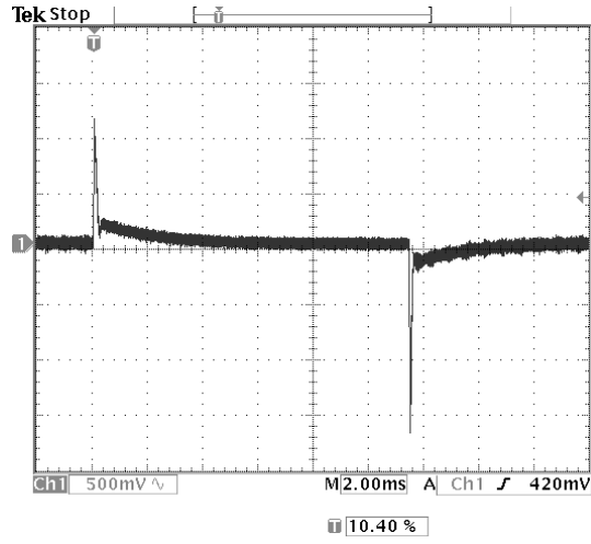
Photo 8: Transient Response 10% to 100% V_{in}=24V , I_{out} = 0.6 to 5.8A C_{out}=1\mu F Ceramic + 10\mu F Tantalum
