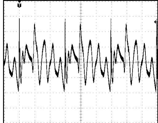
TYPICAL OUTPUT RIPPLE 20mV/div, 1uS/div, full load 75Vin 10uF // 0.1uF decoupling cap room temp
