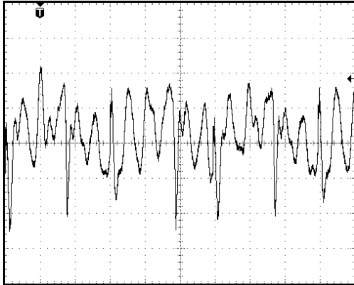
TYPICAL OUTPUT RIPPLE 10mV/div, 1uS/div, full load, 36Vin 10uF // 0.1uF decoupling caps room temp
