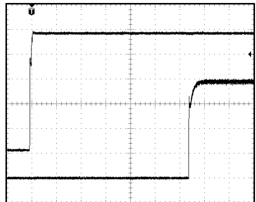
TYPICAL RISE TIME & TURN-ON DELAY WITH Vin 0-48V 500mV/div, 4mS/div (Vout), 10V/div, 4mS/div (Vin) at room temp
