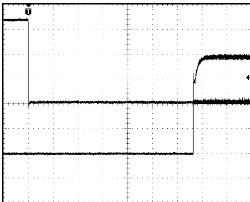
TYPICAL RISE TIME & TURN-ON DELAY USING LOGIC ENABLE 500mV/div, 4mS/div (Vout), 1V/div 4mS/div (logic enable) 36Vin, full load at room temp
