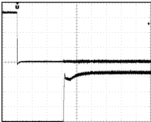
TYPICAL RISE TIME & TURN-ON DELAY USING LOGIC ENABLE 500mV/div, 1mS/div (Vout), 1V/div 1mS/div (logic enable) 36Vin, full load at room temp
