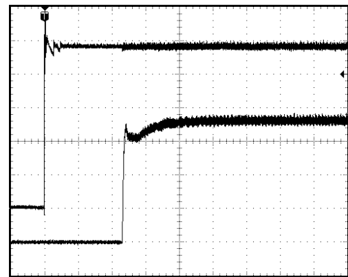
TYPICAL RISE TIME & TURN-ON DELAY WITH Vin 0-48V 500mV/div, 1mS/div (Vout), 10V/div, 1mS/div (Vin) at room temp
