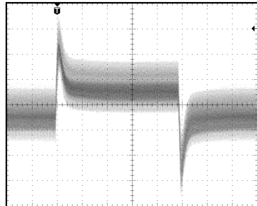
TYPICAL TRANSIENT RESPONSE 20mV/div, 200uS/div, 50% full load to 75% full load 48Vin room temp
