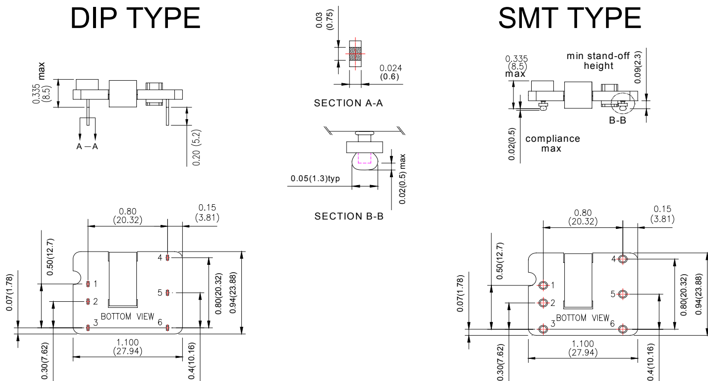
Figure 1: Mechanical Dimensions
