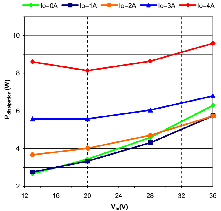
Graph 4: MPQ24S15-50 Power Dissipation vs. Input Voltage
