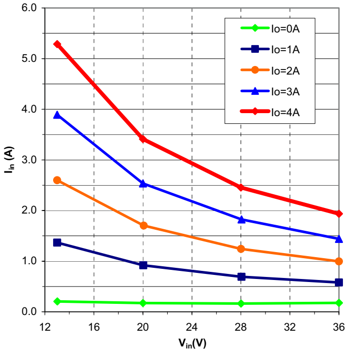
Graph 3: MPQ24S15-50 Input Current vs. Input Voltage
