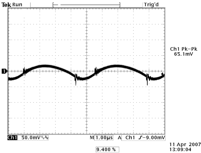
Photo 7: Output Ripple and Noise (20 MHz BW) V_{in}=24\text{ V} , I_{out} = 2.5\text{ A}
