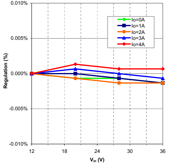
Graph 8: MPQ24S15-50 Line Regulation (+SENSE to +Vout, -SENSE to -Vout)
