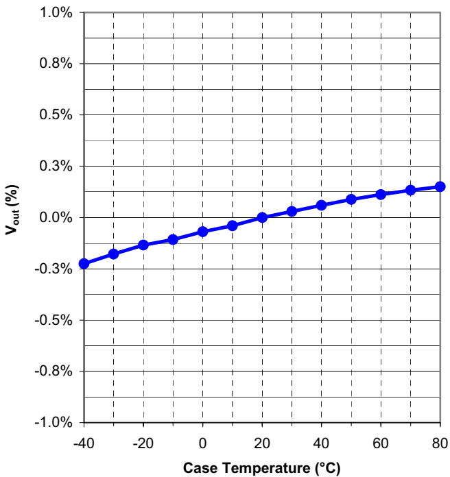
Graph 9: MPQ24S15-50 Output Temperature Drift (+SENSE to +Vout, -SENSE to -Vout)
