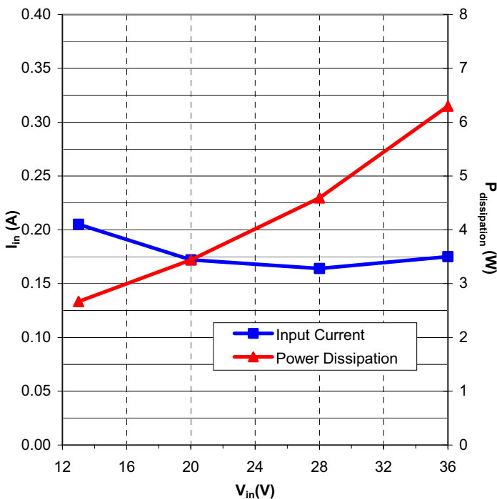
Graph 5: MPQ24S15-50 No Load Input Current and Power Dissipation vs. Input Voltage
