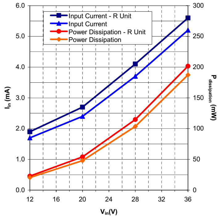
Graph 6: MPQ24S15-50 "Remote Off" Input Current and Power Dissipation vs. Input Voltage
