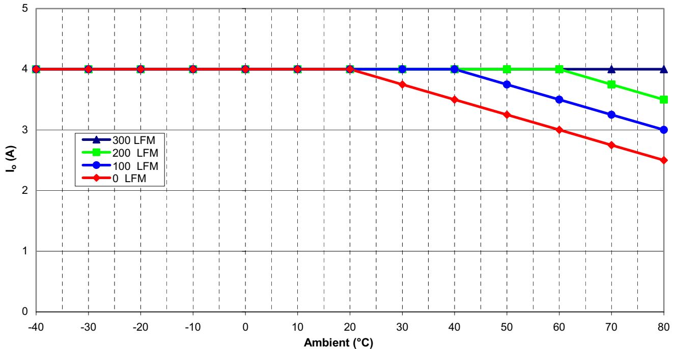
Graph 2: MPQ24S15-50 Max Ambient vs. Io
